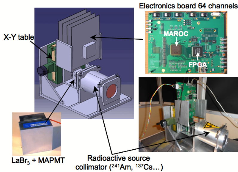
Figure 2: Test bench dedicated to the position resolution measurements.
