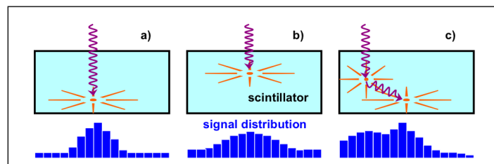
Figure 1: Gamma-ray hit localization in a scintillator coupled to a MAPMT: distributions of scintillation signals for (a) (b) two depths of \gamma -ray photoelectric interaction and (c) a Compton plus photoelectric event.
