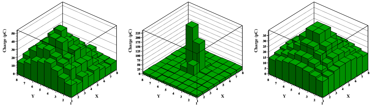
Figure 4: Simulated charge distributions for fully-absorbed 662-keV \gamma -ray irradiation at detector center. Left panel: an event with first hit d.o.i. Z_1 = 1.7 mm and a deposited energy in the first interaction E_1 = 581 keV; middle panel: Z_1 = 18.3 mm and E_1 = 528 keV; right panel: all simulated events.
