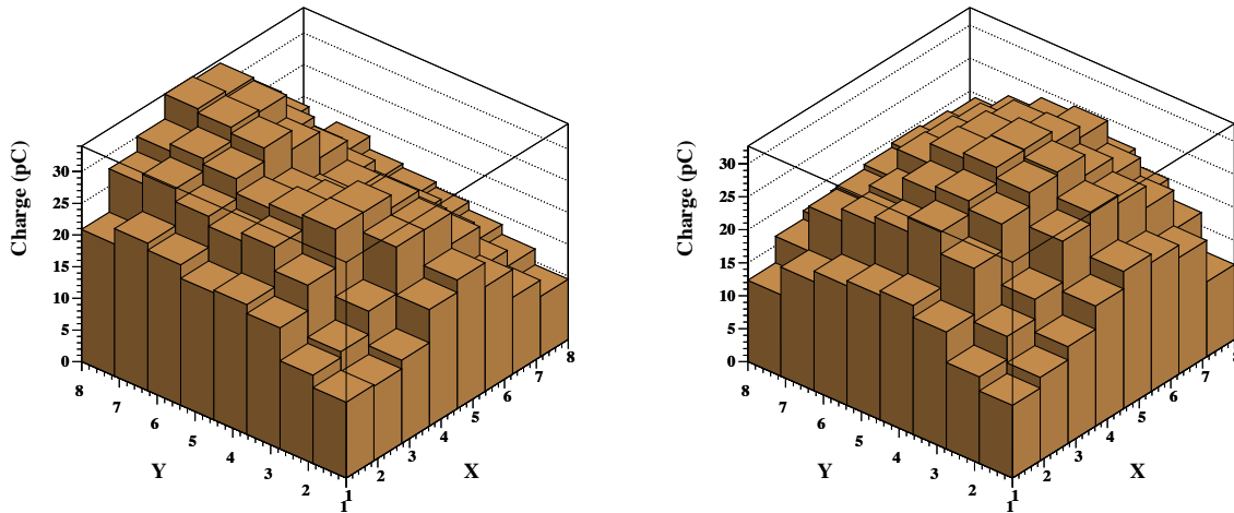
Figure 3: Charge distributions for fully-absorbed 662-keV \gamma -rays measured with a collimated ^{137}\text{Cs} source pointing at the detector centre, before ( left panel ) and after ( right panel ) correction of the non-uniformity of the PMT anodes.
