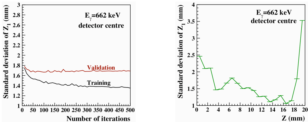
Figure 5: Left panel: mean standard deviation of Z_1 returned by the ANN as a function of the number of iterations in the training process; right panel: standard deviation of Z_1 as a function of the Z -position inside the \text{LaBr}_3 crystal, at iteration 500.
