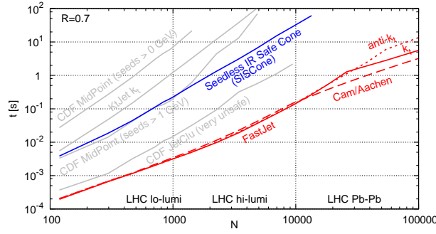
Figure 1: Clustering time as a function of the number of input momenta for several jet algorithms. IR safe algorithms are shown in dark colors (read and blue), and IR unsafe algorithms in light grey. Taken from Ref. [7].
