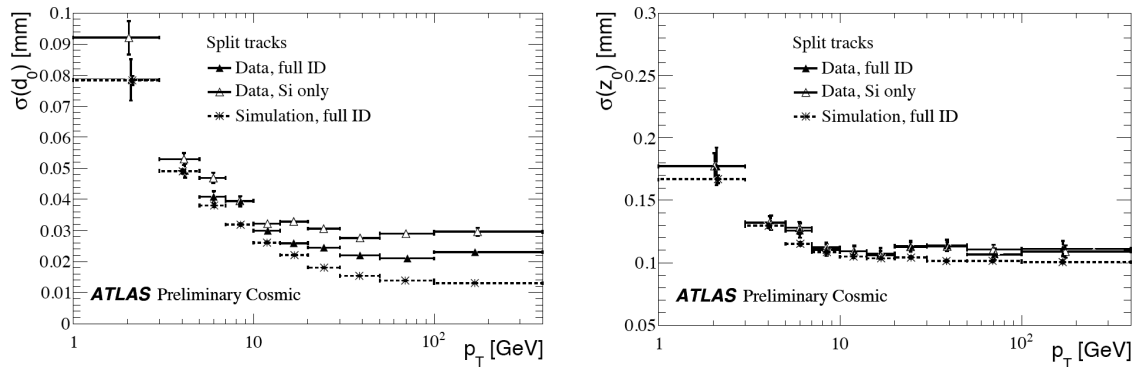
Figure 6: Impact parameter resolutions determined from data and simulation as function of transverse momentum.
