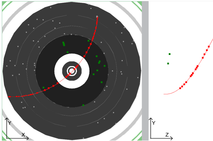
Figure 2: An event display of a reconstructed track (red line) from a cosmic muon producing hits in the Inner Detector (red dots).
