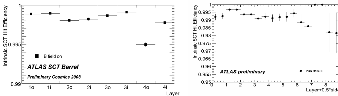
Figure 4: Intrinsic hit efficiencies of the SCT barrel (left) and end-cap (right) as function of barrel layer or end-caps disk and module side.
