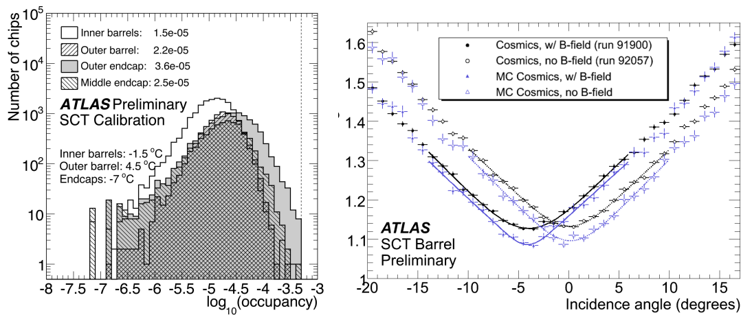
Figure 3: Left plot: noise occupancy of the various barrel and end-cap module types. The dashed line represents the specification limit. Right plot: the Lorentz angle measurement with and without magnetic field obtained from data and simulation.
