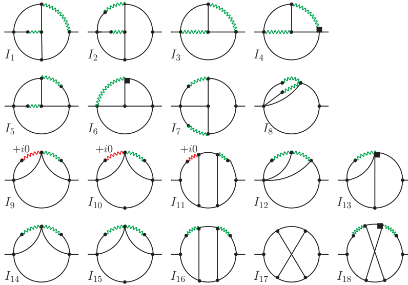
Figure 1: Most complicated master integrals contributing to a_3 . The solid and zig-zag lines correspond to relativistic and static propagators, respectively. Small black boxes denote monomials in numerators.
