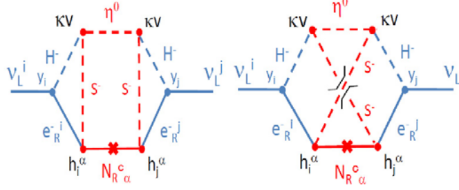
Figure 1: The diagrams for generating tiny neutrino masses.
