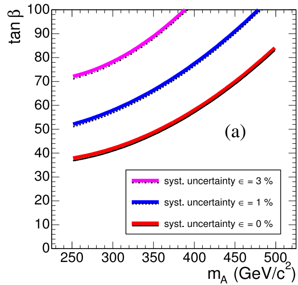
Figure 2: The 5\sigma -discovery region in the m_A , \tan\beta plane for charged Higgs bosons with the H^\pm \rightarrow tb decay channel for 30 \text{ fb}^{-1} assuming precise knowledge of the background (solid line) and a systematic uncertainties of 1% (dashed line) and 3% (dash-dotted line).
