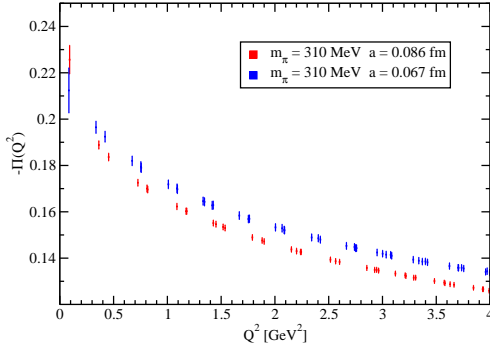
Figure 5: Lattice spacing dependence of -\pi(q^2) . The unrenormalized -\pi(q^2) is shown. The discrepancy illustrates the ultra-violet subtraction required to renormalize \pi .
