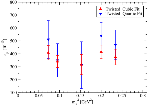
Figure 9: Comparison of cubic and quartic fit results for a_\mu^{\text{had}} . There is general agreement between the cubic and quartic fits for all calculations excluding the smaller volume at m_\pi = 310 MeV (not shown).
