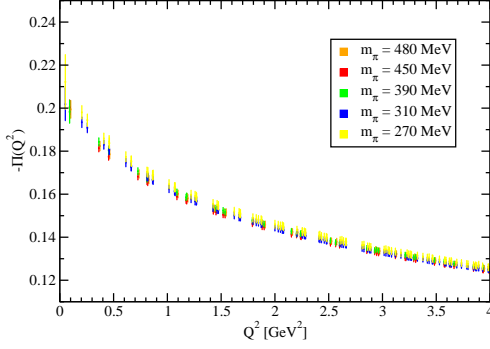
Figure 3: Quark mass dependence at large q^2 . There is no noticeable quark mass dependence at large q^2 , consistent with perturbative QCD expectations.
