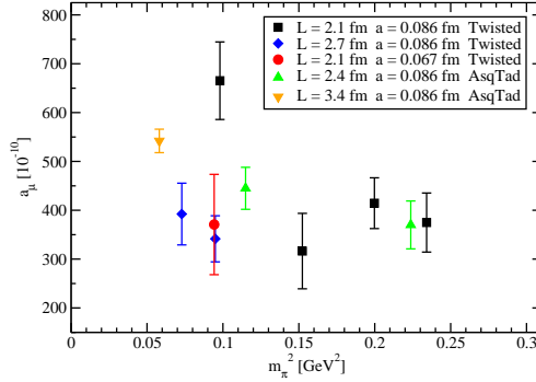
Figure 10: Comparison of all full QCD calculations of a_\mu^{\text{had}} . The results of this work are shown along with the staggered results of [11]. Finite size effects and lattice artifacts are visible.
