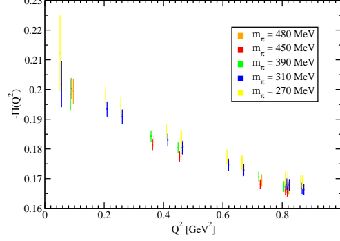
Figure 4: Quark mass dependence at low q^2 . There is a systematic, but not statistically significant, shift with quark mass from m_\pi = 450 MeV to 270 MeV.
