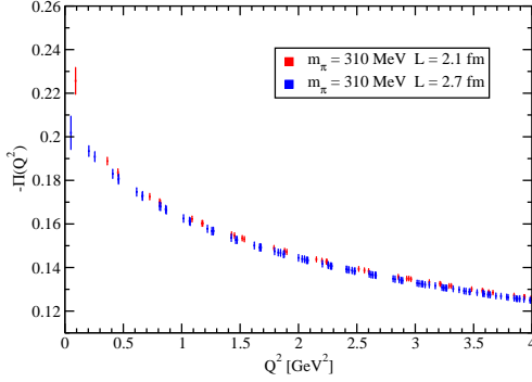
Figure 1: Volume dependence of -\pi(q^2) . This quantity requires an ultra-violet subtraction but is infra-red finite. With the exception of the lowest q^2 point, there is no noticeable finite size effect.
