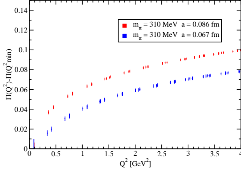
Figure 7: Lattice spacing dependence of \pi(q^2) - \pi(0) . The results have been renormalized at the lowest value of q^2 at each lattice spacing to illustrate the effect of the subtraction.
