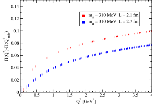
Figure 2: Volume dependence of \pi(q^2) - \pi(0) . As an illustration, this quantity is renormalized at the lowest momentum accessible in each volume, demonstrating the sensitive nature of the subtraction.
