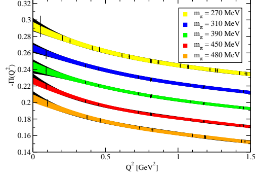
Figure 8: Low q^2 extrapolation. Each \pi(q^2) has been fit to cubic (foreground) and quartic (background) functions of q^2 , showing agreement for all but the smaller volume at 310 MeV (not shown).
