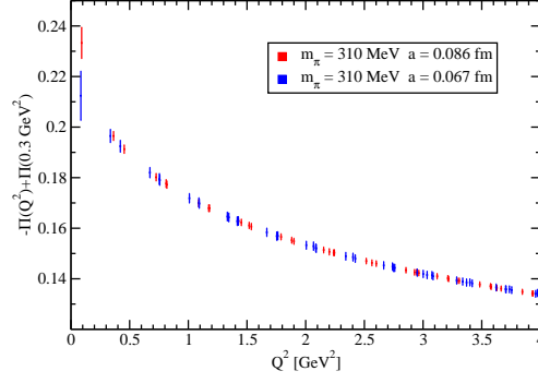
Figure 6: Lattice spacing dependence of -\pi(q^2) matched at q^2 = 0.3 GeV 2 . With the exception of the lowest q^2 point, there is no noticeable lattice spacing dependence.
