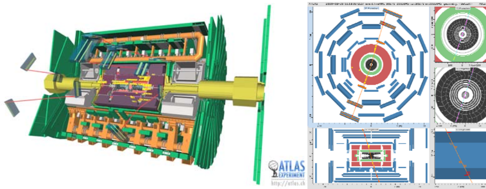
Figure 4: Left: beam-halo event from single LHC beam operation on 10th September 2008. Right: cosmic ray muon traversing the full ATLAS detector.
