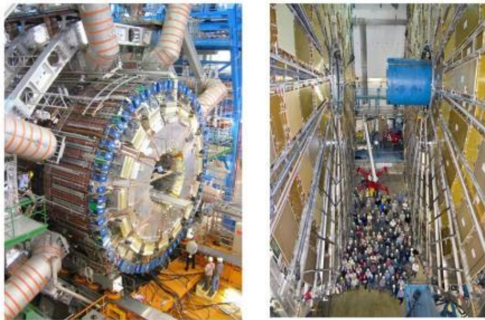
Figure 2: Left: the barrel calorimeter being moved into position inside the toroid in November 2005. Right: the large end-cap muon wheels after completion of the installation in September 2007.
