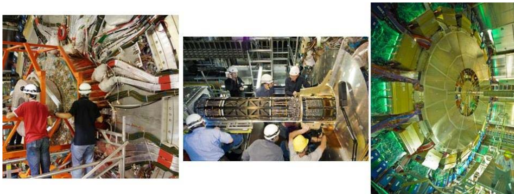
Figure 3: Left: the barrel TRT and SCT being installed in August 2006. Middle: the Pixel detector being inserted in June 2007. Right: ID volume sealed with the end-plate in April 2008.
