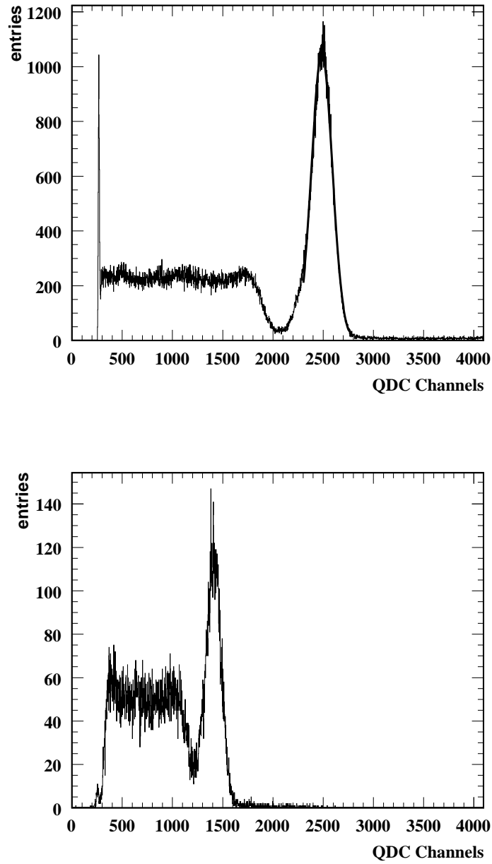
Figure 2: Energy response to a ^{22}\text{Na} source of (a) 3 \times 3 \times 15 \text{ mm}^3 LSO crystal coupled with a 3 \times 3 \text{ mm}^2 MPPC (3600 pixels) and (b) 1 \times 1 \times 15 \text{ mm}^3 LSO crystal coupled with a 1 \times 1 \text{ mm}^2 MPPC (400 pixels).
