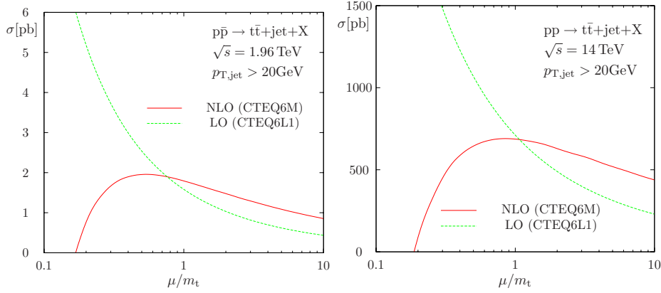
Figure 1: Scale dependence of the LO and NLO cross sections for t\bar{t} + \text{jet} production at the Tevatron (left) and at the LHC (right) as taken from Ref. [6], where the renormalization scale ( \mu_r ) and the factorization scale ( \mu_f ) are set equal to \mu .
