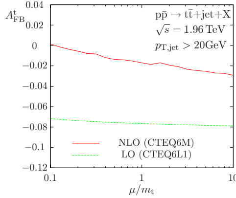
Figure 2: Scale dependence of the LO and NLO forward-backward charge asymmetry of the top quark in p\bar{p} \rightarrow t\bar{t} + \text{jet} + X at the Tevatron as taken from Ref. [6] with \mu = \mu_f = \mu_r .
