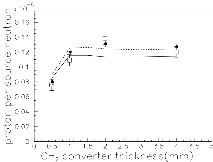
Figure 4: Proton to neutron conversion ratios deduced from the measurements (open squares), from the simulations (dashed line) and from the simulations with a 1.5 MeV energy threshold associated to silicon 3 detector (solid line). The conversion ratios deduced from the scaler values read during the experiment are also plotted (filled circles).
