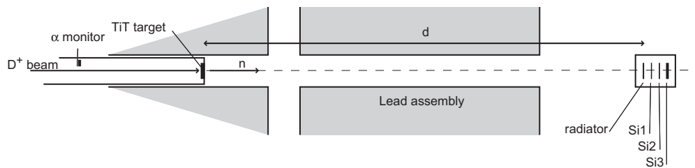
Figure 1: Experiment set-up.
