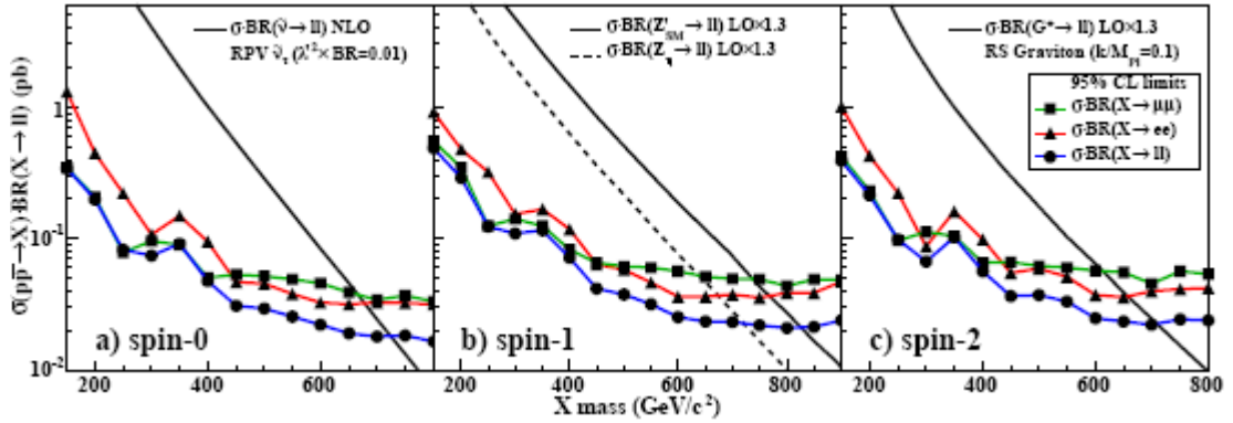
Figure 1. The \sigma(X_{ll}) limits from ee , \mu\mu and combined s channels as a function of m_X for spin-0 (a), spin-1 (b), and spin-2 (c). Also shown are theoretical predictions of representative models.
