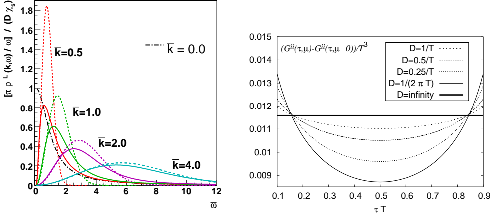
Figure 2: The low energy longitudinal spectral function \rho_{\text{low}}^L(\mathbf{k}, \omega, T) (left) and the low energy contribution to the correlator (right). Here \bar{\omega} = \omega(M/T) and \bar{k} = kD\sqrt{M/T} .
