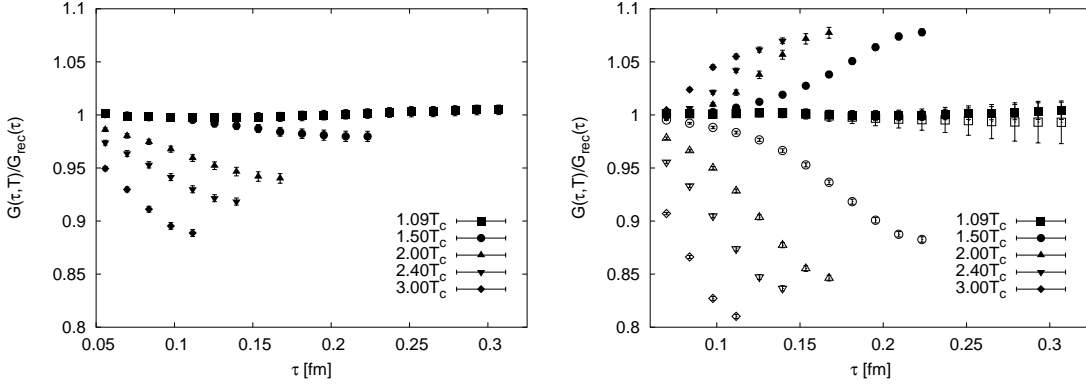
Figure 1: The ratio G/G_{\text{rec}} for pseudo-scalar (left) and vector (right) channels at \mathbf{k} = 0 . For the vector case we show both the sum over spatial components (filled symbols) and all four components (open symbols).
