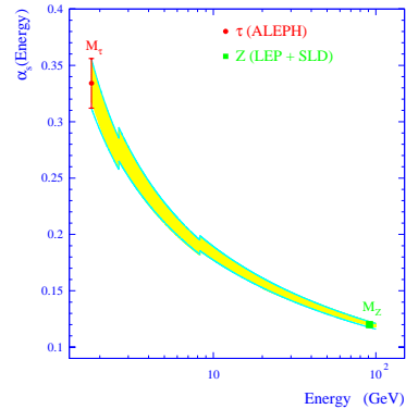
Figure 10: Evolution of the strong coupling (measured at m_\tau^2 ) to M_Z^2 predicted by QCD compared to the direct measurement. The evolution is carried out at 4 loops, while the flavour matching is accomplished at 3 loops at 2 m_c and 2 m_b thresholds.
