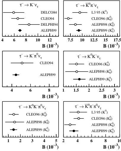
Figure 15: Some of the new ALEPH results on decay modes with kaons compared to the published data.
