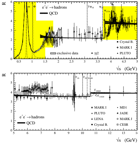
Figure 12: Inclusive hadronic cross section ratio in e^+e^- annihilation versus the c.m. energy \sqrt{s} . Additionally shown is the QCD prediction of the continuum contribution from reference [28] as explained in the text. The shaded areas depict regions where experimental data are used for the evaluation of \Delta\alpha_{\text{had}}(M_Z^2) and a_\mu^{\text{had}} in addition to the measured narrow resonance parameters. The exclusive e^+e^- cross section measurements at low c.m. energies are taken from DM1,DM2,M2N,M3N,OLYA,CMD,ND and \tau data from ALEPH (see reference [10] for detailed information).
