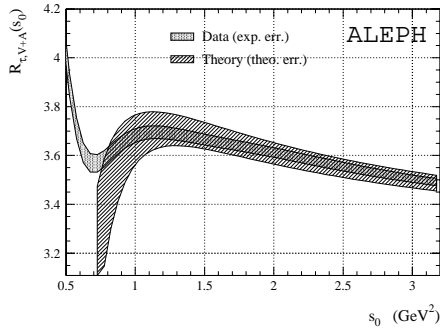
Figure 8: The ratio R_{\tau, V+A} versus the square “ \tau mass” s_0 . The curves are plotted as error bands to emphasize their strong point-to-point correlations in s_0 . Also shown is the theoretical prediction using the results of the fit at s_0 = m_\tau^2 .
