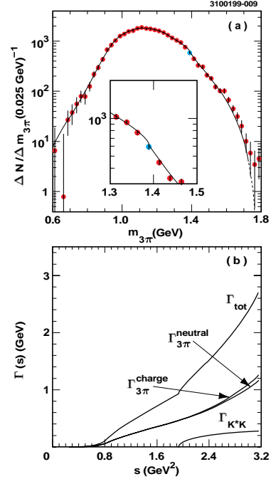
Figure 4: (a) 3\pi mass spectrum from CLEO in the \pi^- 2\pi^0 channel with the lineshape from the resonance fit (zoom on the K^*K threshold). In (b), the \sqrt{s} -dependent a_1 width is plotted with the different contributions considered.
