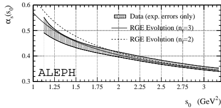
Figure 9: The running of \alpha_s(s_0) obtained from the fit of the theoretical prediction to R_{\tau, V+A}(s_0) . The shaded band shows the data including experimental errors. The curves give the four-loop RGE evolution for two and three flavours.
