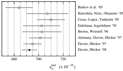
Figure 14: Comparison of a_\mu^{\text{had}} evaluations. The values are taken from references [47, 48, 49, 37, 50, 10, 28, 30].
