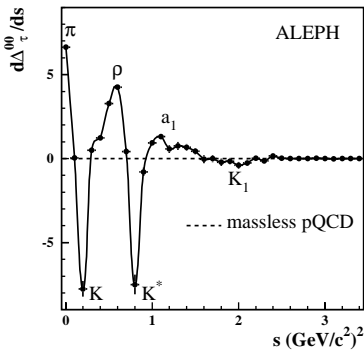
Figure 17: Integrand of equation (6.5) for (k=0, l=0) , i.e. , difference of the Cabibbo-corrected non-strange and strange invariant mass spectra.
