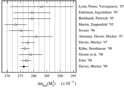
Figure 13: Comparison of \Delta\alpha_{\text{had}}(M_Z^2) evaluations. The values are taken from references [41, 37, 42, 43, 44, 10, 28, 45, 46, 30].
